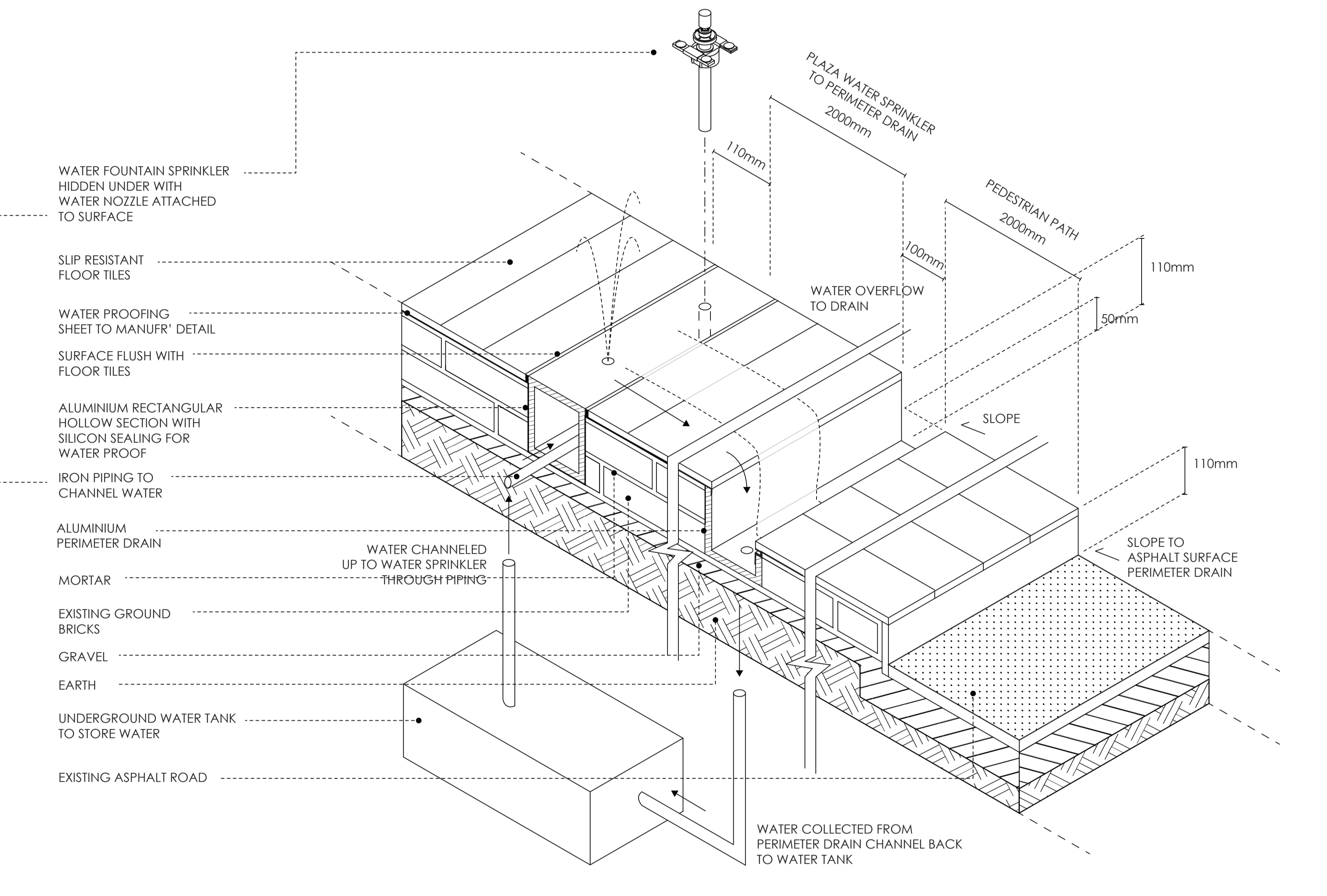
WATER FOUNTAIN PLAZA, PEDESTRIAN PAVEMENT AND ASPHALT ROAD CONNECTION DETAILS 0 200mm SCALE 1:5
