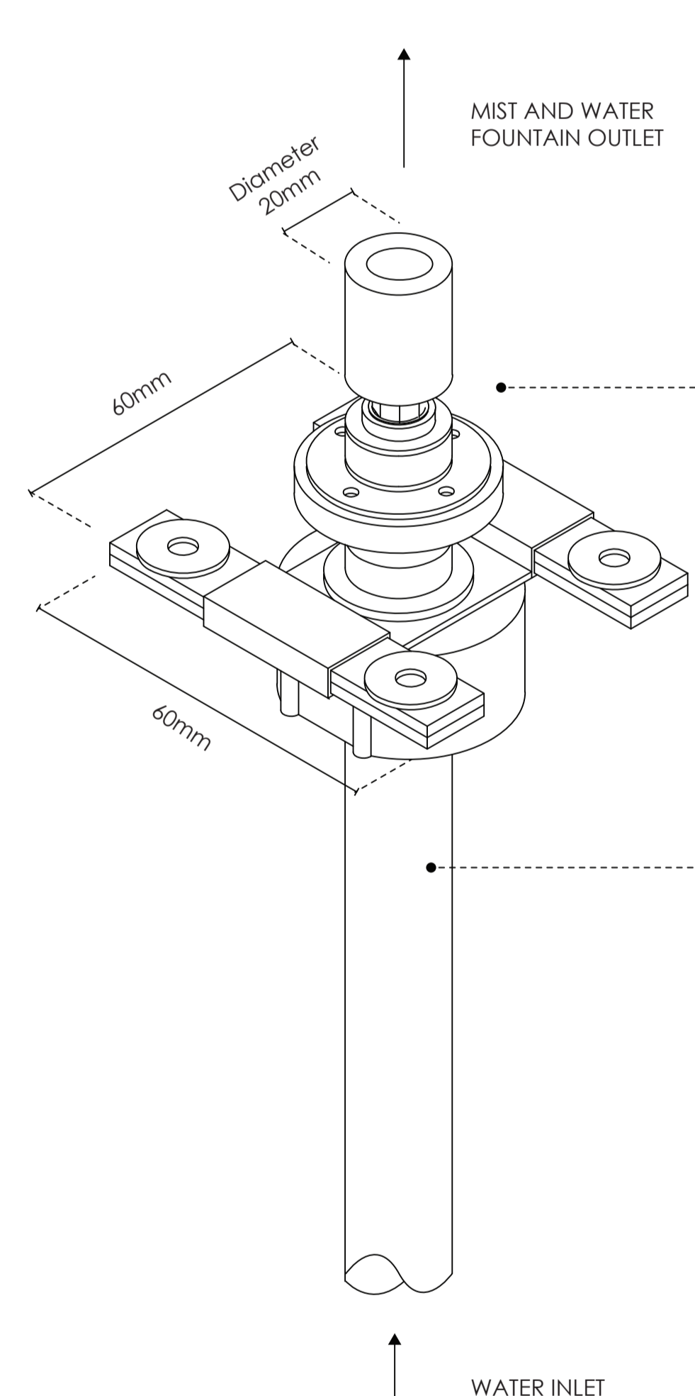
WATER FOUNTAIN SPRINKLER 2 IN 1 MIST & WATER SPRINKLER TO MANUFACTURER'S DETAIL 0 50mm SCALE 1:1
